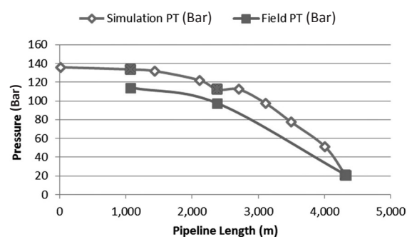
Figure 7: Field Data Vs Simulation Result Comparison (Pressure).
