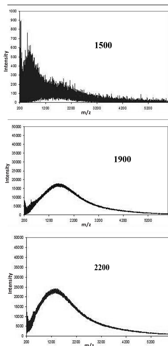
Figure 3: Sequences of LDIMS of asphaltenes (Furrial) measured at increasing LS power. The increase in LS apparently promotes both fragmentation and ring fusion, as suggested by the observed large MMD changes observed in this LS range (200-5200 amu range).
