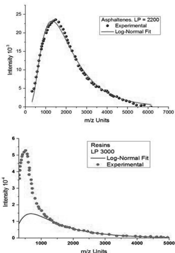
Figure 8: Fitting a log-normal distribution (Equation 10) to experimental data for the asphaltenes (top) and the resins (bottom) at the shown laser power. Apparent conversion to FPAH's is complete for the asphaltenes and partial (approximately 60%) in the case of the resins.
