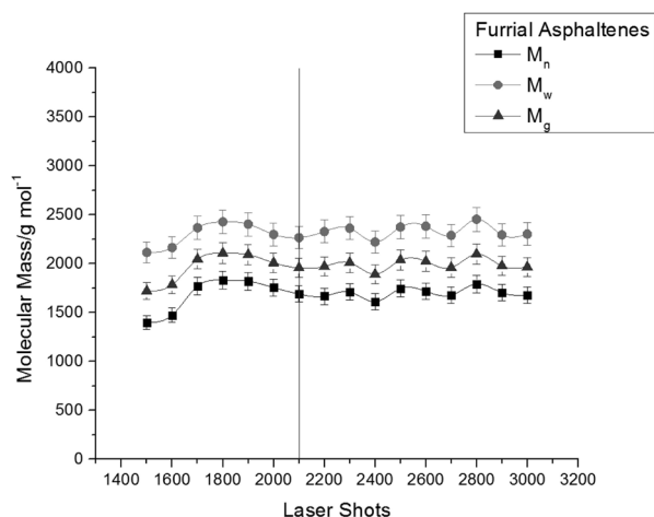
Figure 7: Dependence of the molecular mass on LS for Furrial asphaltenes. The maximum below LS = 2100 is consistent with the simultaneous operation of ring fusion and fragmentation, which have opposite effects on the sample mass. The sector to the right of LS = 2100 corresponds to fullerene formation and the loss of hydrogen and other elements.
