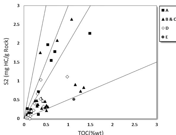
Figure 7: S2 versus TOC in middle Sarvak [29].
