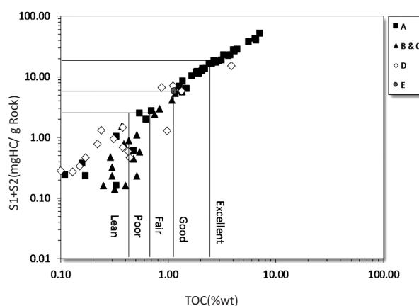
Figure 5: S 1 +S 2 versus TOC in the middle Sarvak formation [27].
