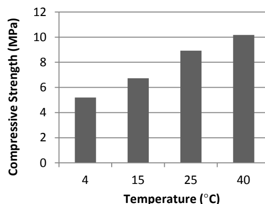
Figure 2: Effect of temperature on compressive strength [1].
