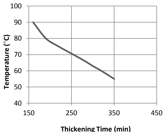
Figure 1: Effect of temperature on thickening time of cement class G with 2% \text{CaCl}_2 [1, 2].
