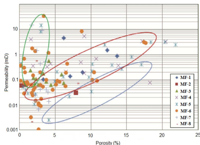
Fig. 13 Relationships between various microfacies and HFU's in the studied interval of Fahliyan Formation.
