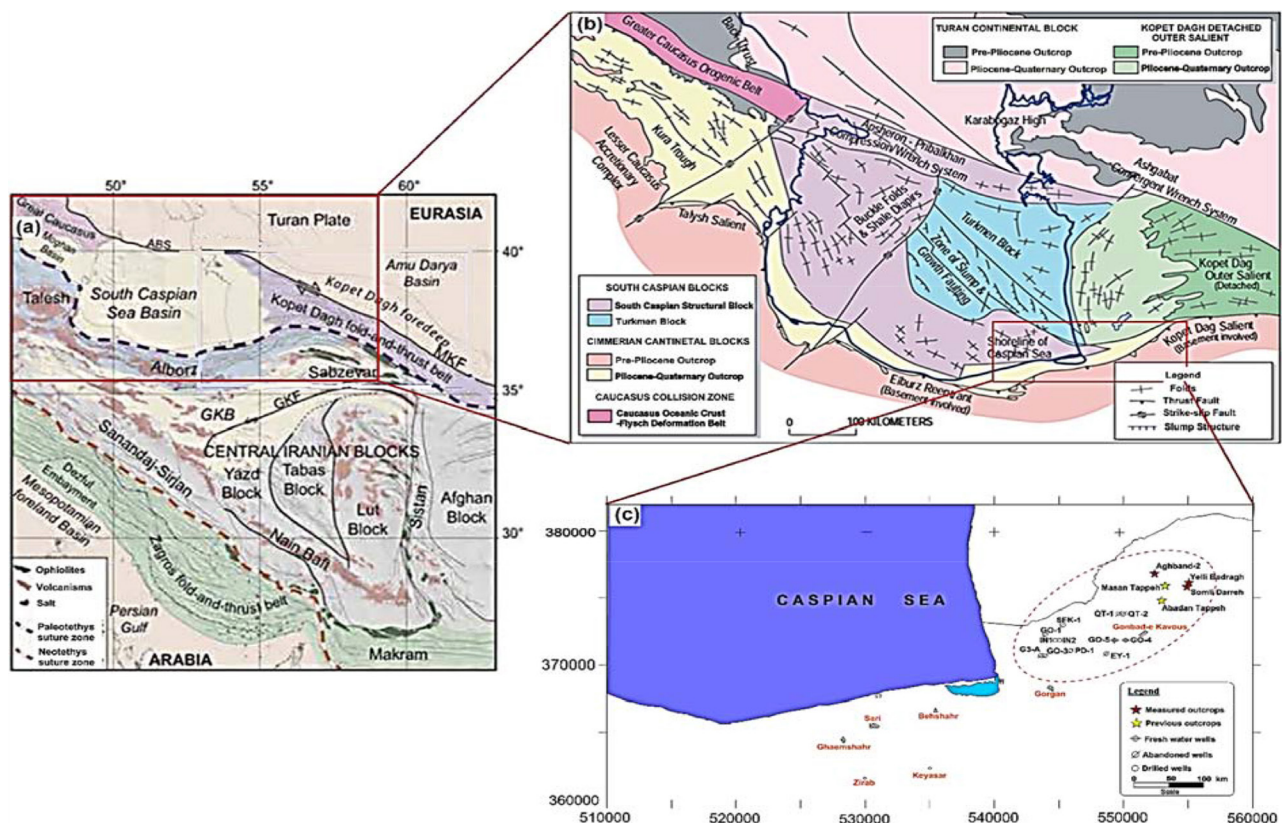
Fig 1: (a) Map of the different zones and main structural divisions of Iran [11], (b) Major structural blocks in the South Caspian Basin [12], location of the study area outlined in a red rectangle. (c) The outcrops are shown in a red dashed curve along with the subsurface sections in northeastern Iran.
