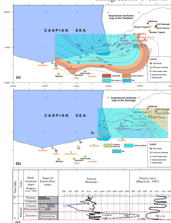
Fig 6: (a and b) Isopach/ Isolith map of the Cheleken and Akchagyl Formations, (c) Main sea-level fluctuations of the Mediterranean [35] and Eastern Para-Tethys [30] compared with the eustacy curve [36] during the Early (Zanclean stage, red dashed rectangle) to Late (Piacenzian- Gelasian stages, blue dashed rectangle) Pliocene. The curve of sea-level fluctuations in the Caspian Basin is shown with a dashed curve.
